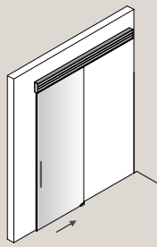
A parete / Wall mounted L min 135 max 600 cm W min 53.15" max 236.22"
