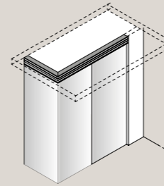
Pannello fisso soffitto / Ceiling mounted fixed panel
