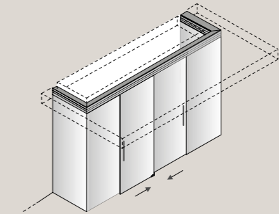
2 pannelli fissi e 2 ante su binario birotaia a soffitto / 2 fixed panels and 2 doors on recessed double track
