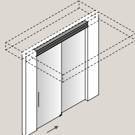
Ad incasso / Recessed L min 138 max 600 cm W min 54.33" max 236.22"
