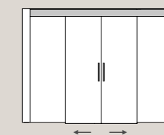
2 ante scorrevoli e 2 pannelli fissi binario a soffitto / 2 sliding doors and 2 fixed panels on a ceiling mounted track
